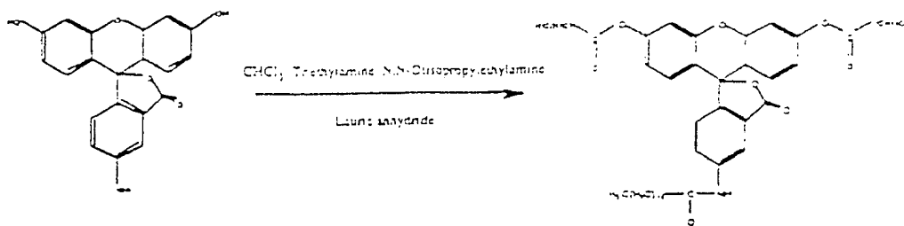
Synthesis of 5-dodecanoyl-aminofluorescein-di-dodecanoic acid
